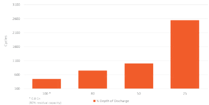
GEL Cycle Life vs Depth of Discharge at +25°C Based on EN60254-1
